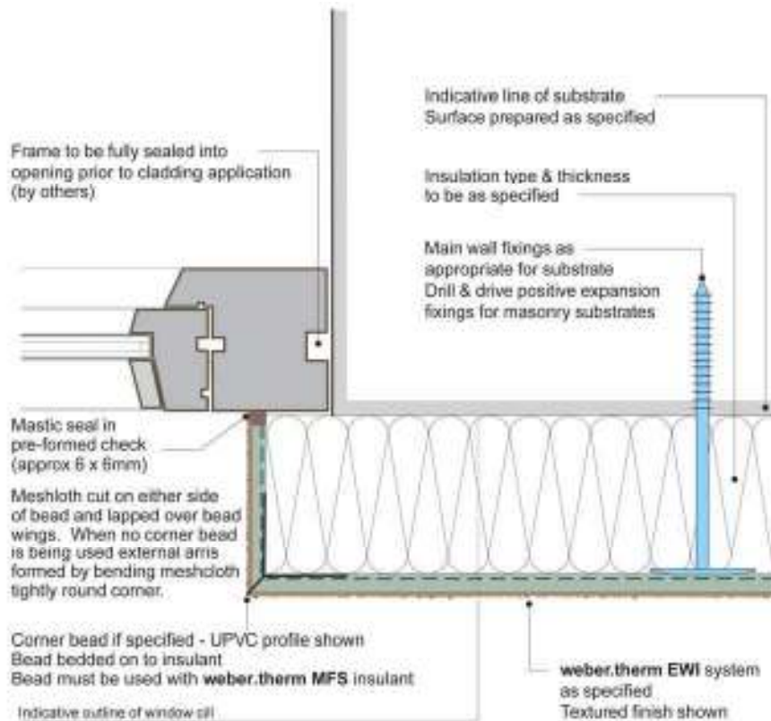
Figure 4: Window Reveal
