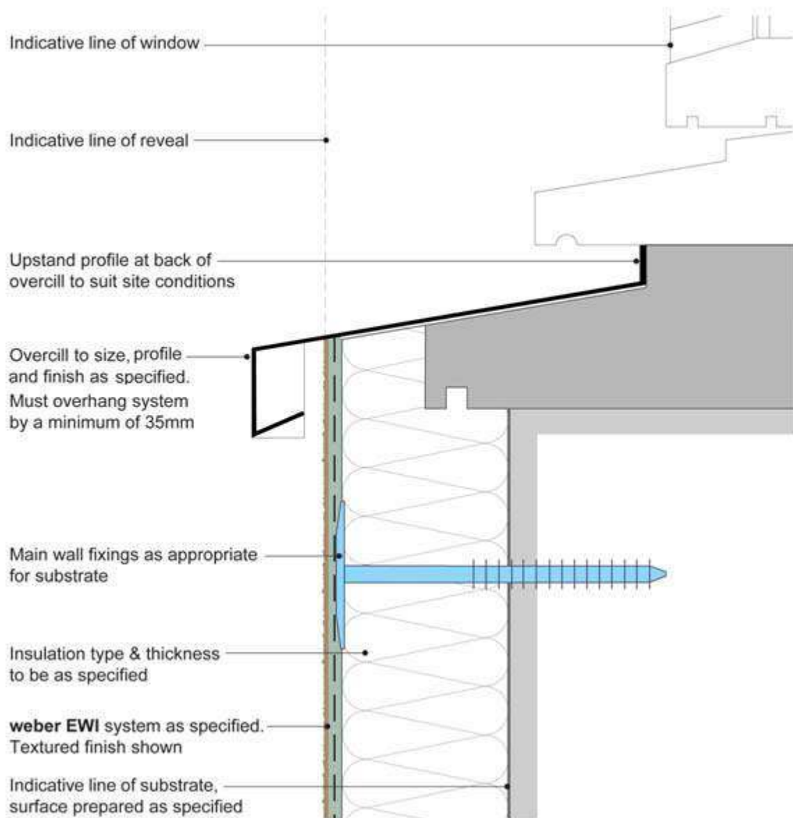
Figure 12: Window Sill
